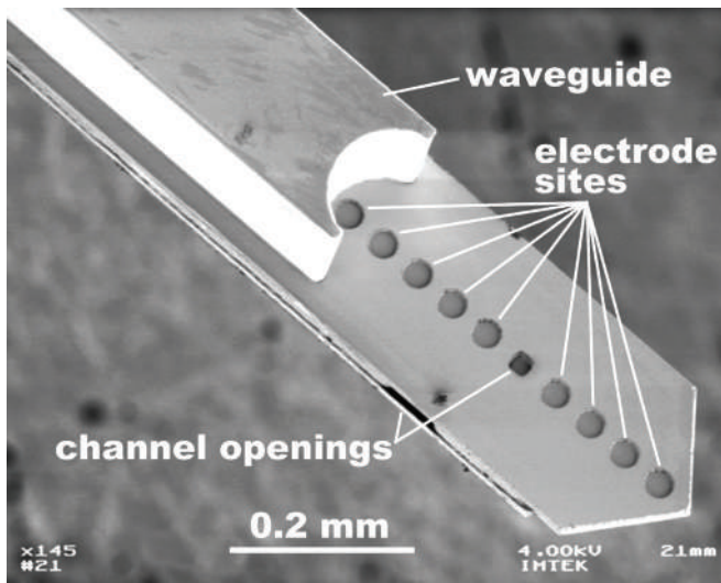
Scanning electron micrograph of a multimodal shaft's tip. The picture shows nine platinum electrode sites (circular openings) for the measurement of electrical signals, injection channels for fluids (rectangular openings), and a concave waveguide for optical stimulation.
